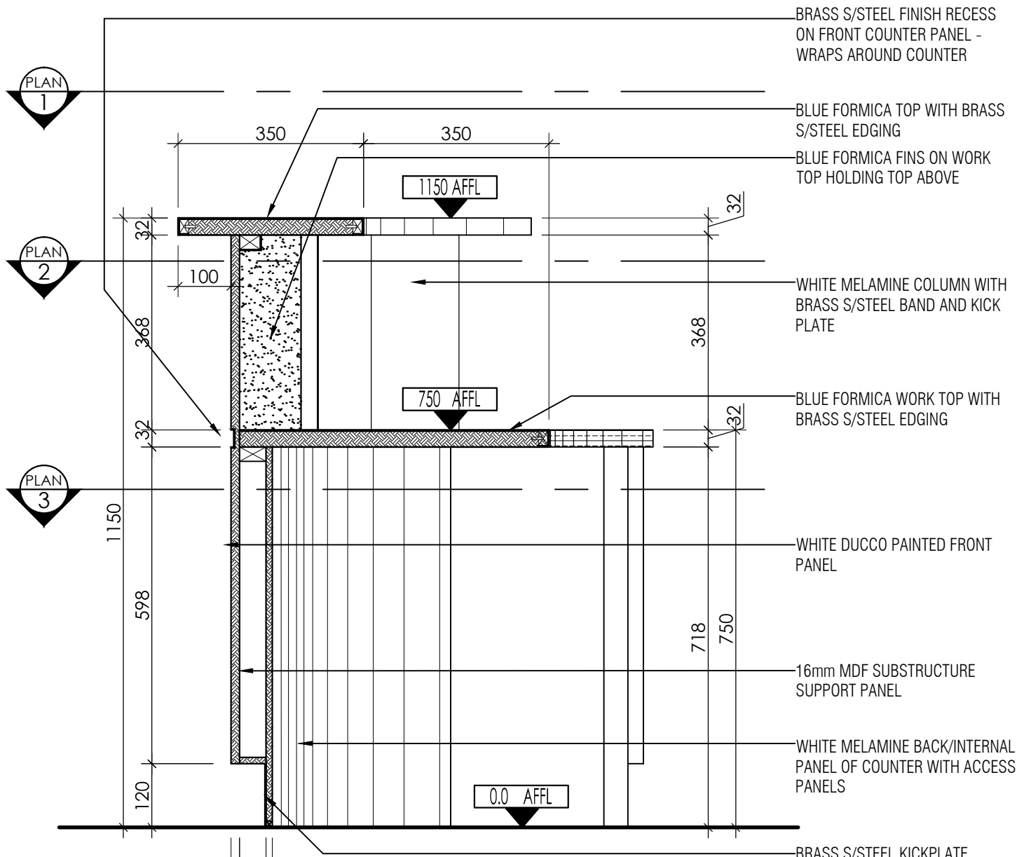
RECEPTION DESK SECTION A-A Scale 1:10
